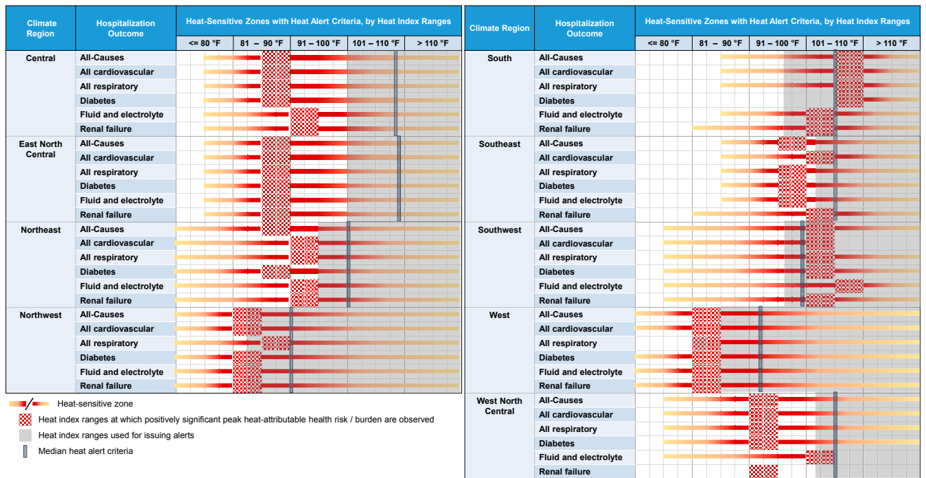
Fig. 3. Region-specific heat-sensitive zones with heat alert criteria.
